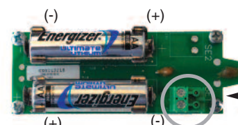
Fig. 2-6 WIRE CONNECTION TO TERMINAL BLOCK
